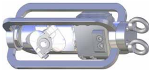
Type L 1400-2 with sledge for cleaning pipes with bends 35 mm S-arm, 2 nozzles max. 1400 bar / 150 l/min. Min. Pipe -Ø: 210 mm
